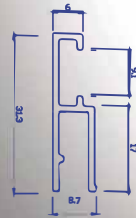
H Profile
