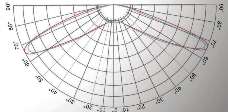
Latitudinal ( Vertical Angle ) Polar Radiation Pattern
