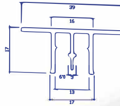
W Profile
