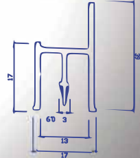
M Profile
