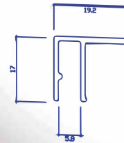
F Profile
